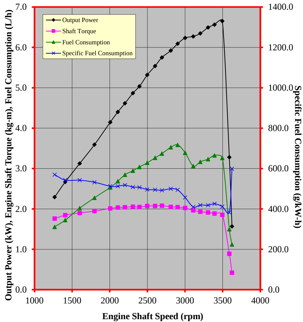
Figure 3. Performance characteristic curves of the KINGSTAR 189F Diesel Engine
