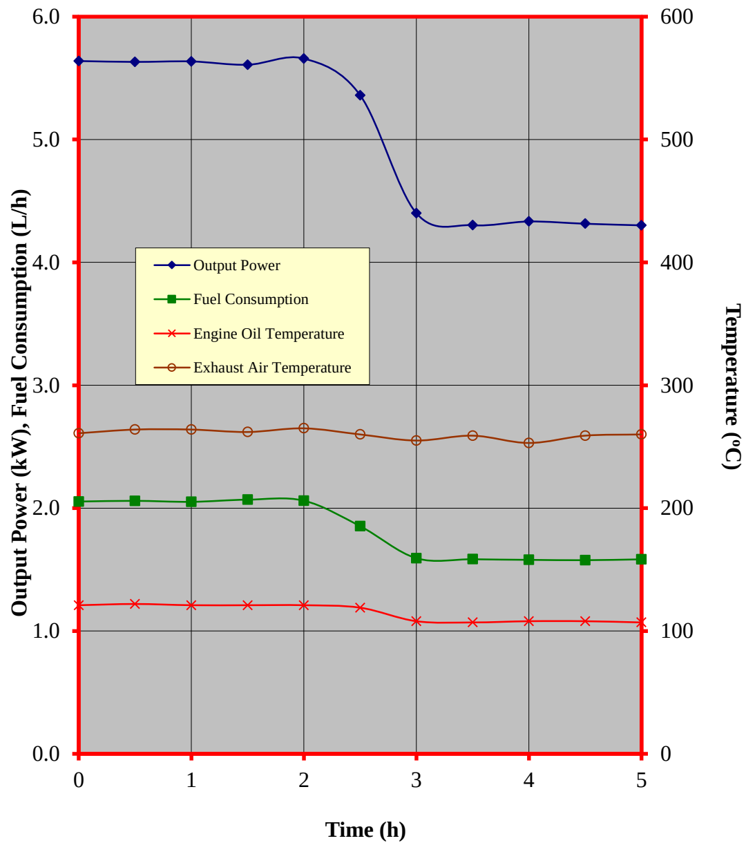
Figure 4. Performance characteristic curves during the continuous running test of the KINGSTAR 189F(E) Diesel Engine
